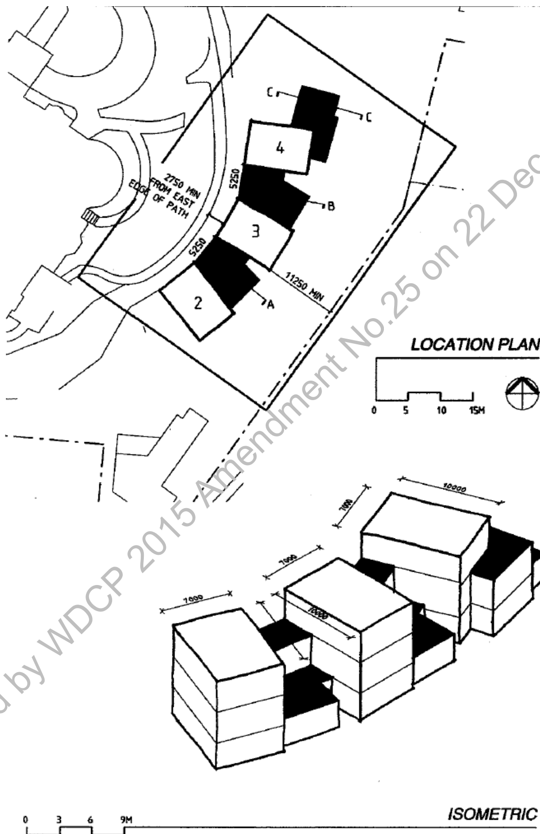
FIGURE 11 B2 to B4 – Building envelope diagram (location and isometric)
