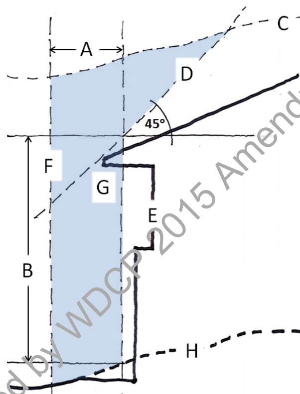
FIGURE 8 Section view of the building envelope with the setbacks and inclined plane A = Side setback B = 7.2m maximum wall height C = Maximum building height: 9.5m above existing ground level D = Inclined plane: 45degrees to horizontal E = Potential built form F = Site boundary G = Roof eaves may protrude into the setback if below the inclined plane H = Existing ground level
