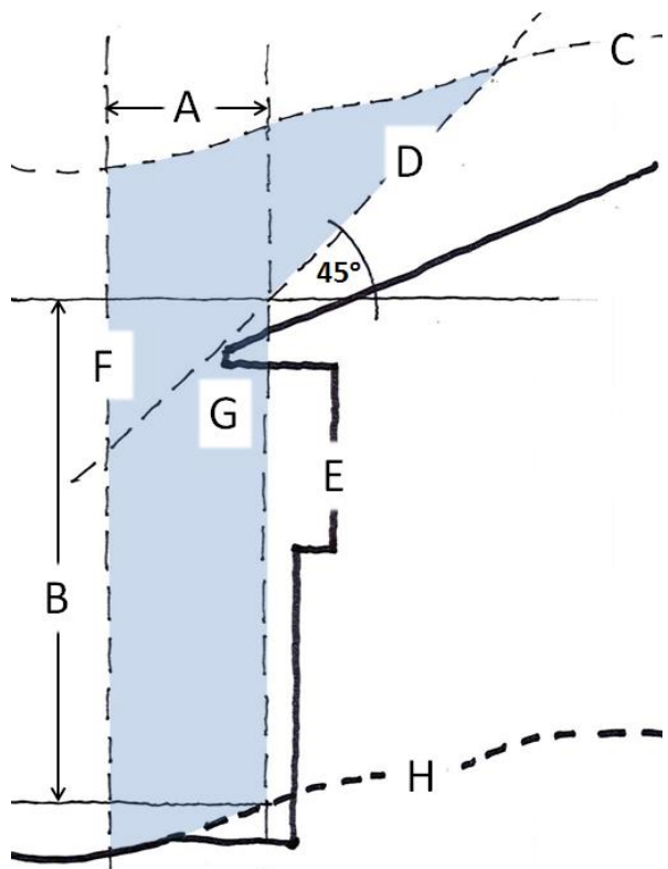
FIGURE 9 Section view of the building envelope with the setbacks and inclined plane A = Side setback B = 7.2m maximum wall height C = Maximum building height: 9.5m above existing ground level D = Inclined plane: 45degrees to horizontal E = Potential built form F = Site boundary G = Roof eaves may protrude into the setback if below the inclined plane H = Existing ground level
