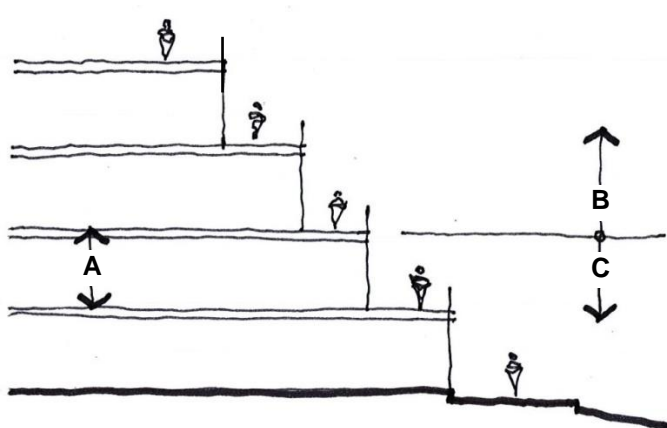
FIGURE 19 Application of the visual privacy controls to roof terraces A - Second storey B - Refer to B3.5.4 C10 C - Refer to B3.5.4 C7
