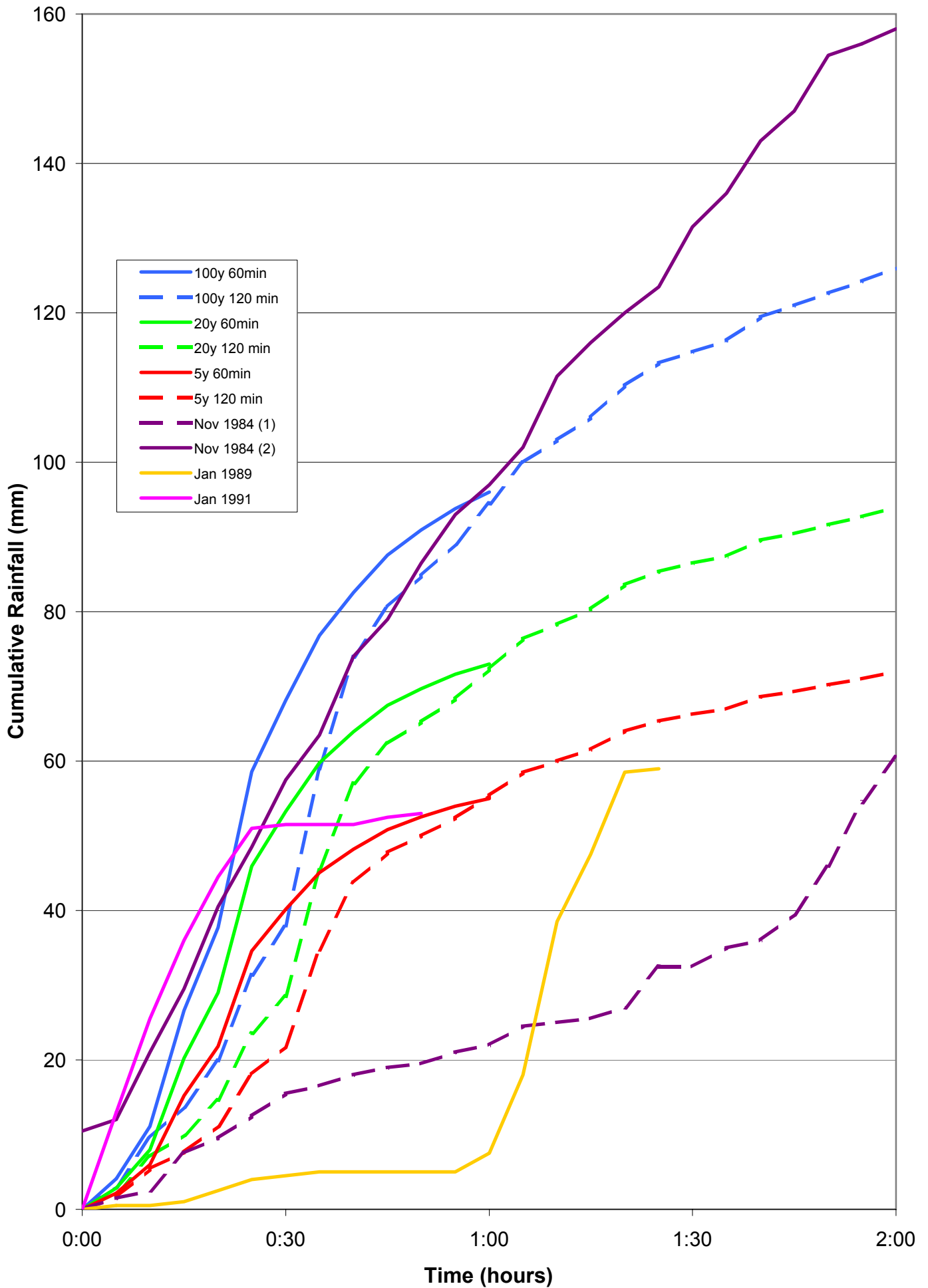
FIGURE 2 COMPARISON OF DESIGN AND HISTORICAL RAINFALL
