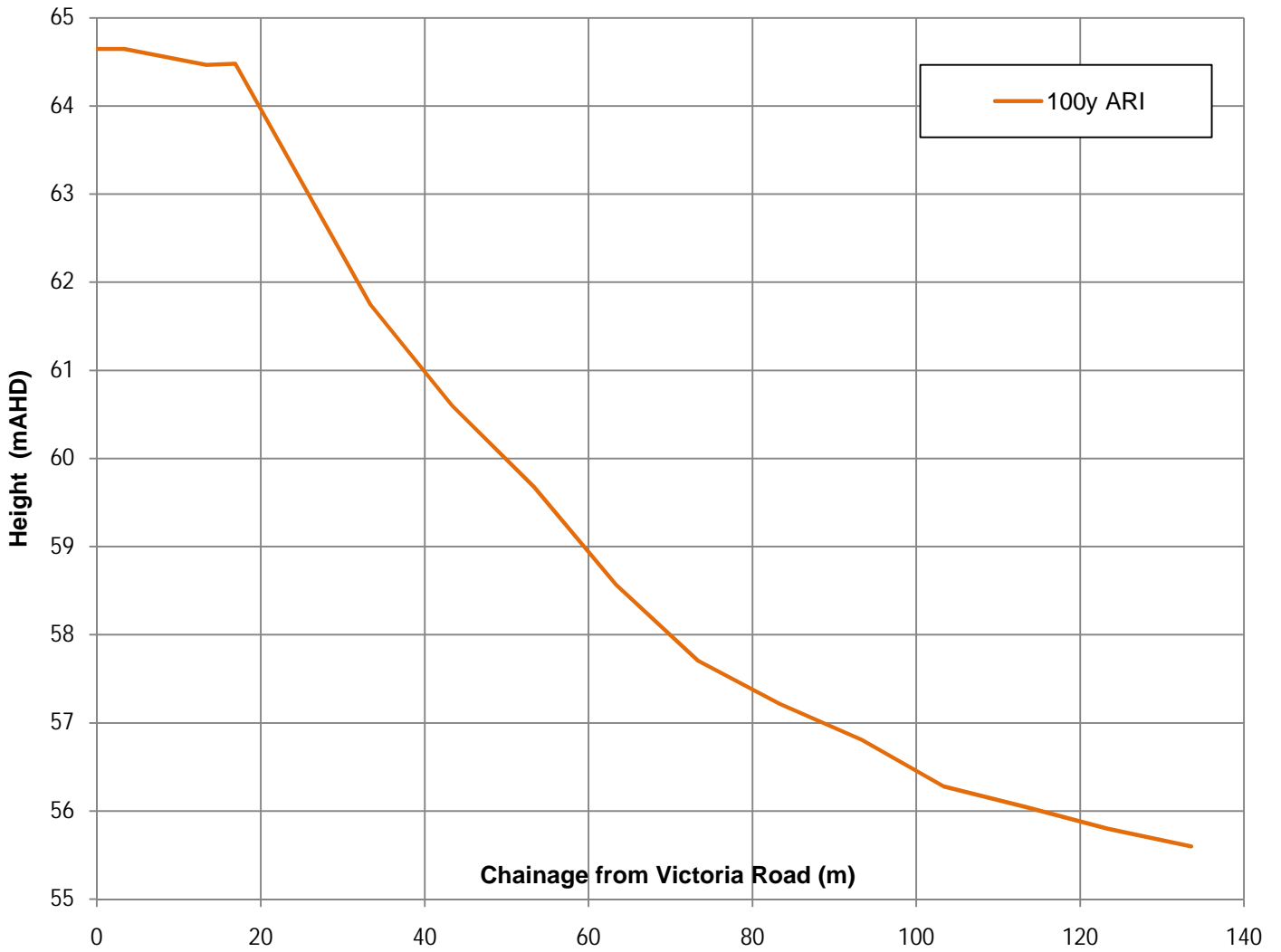
FIGURE 7i PEAK HEIGHT PROFILES REACH 9
