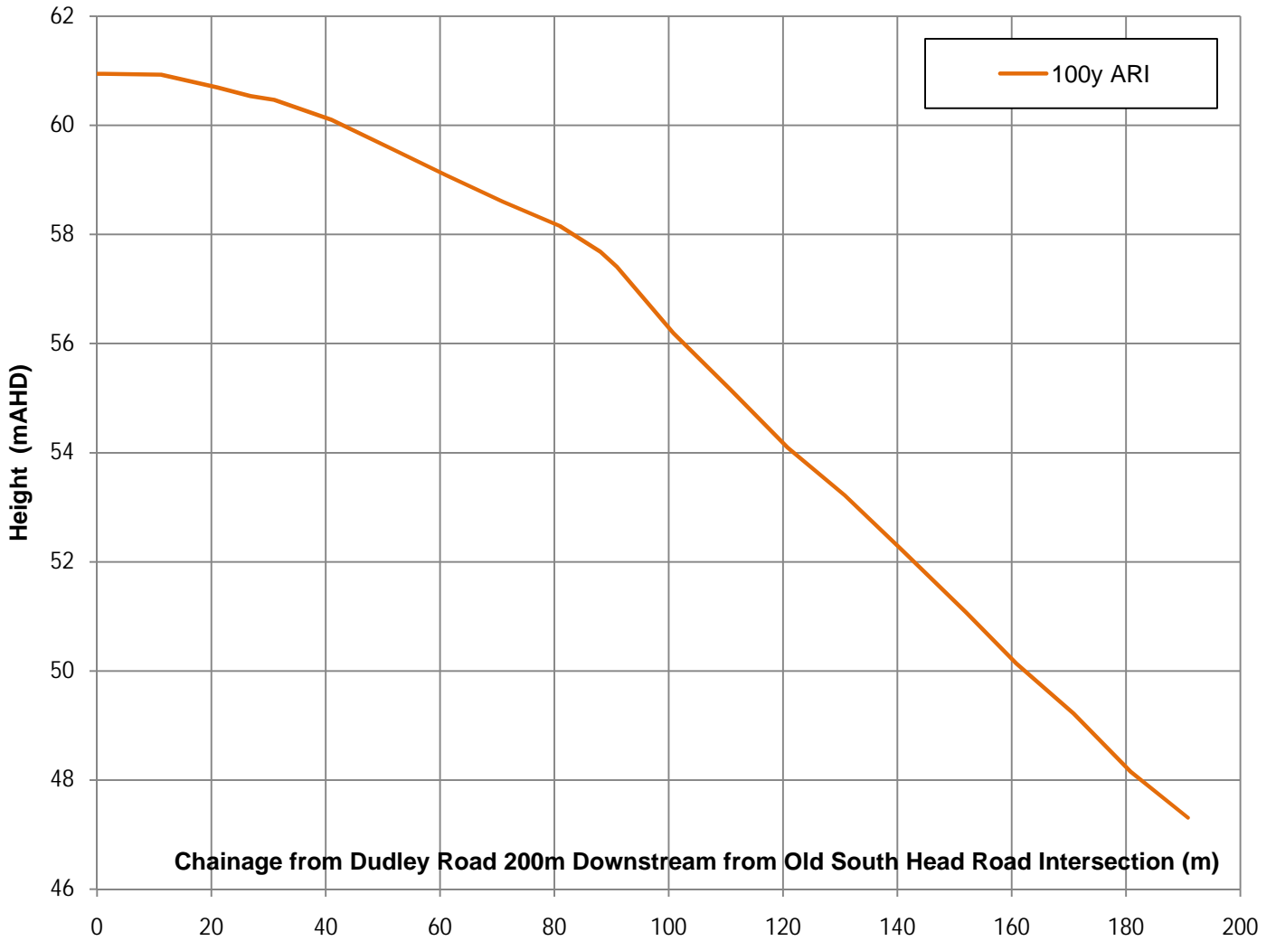
FIGURE 7b PEAK HEIGHT PROFILES REACH 2
