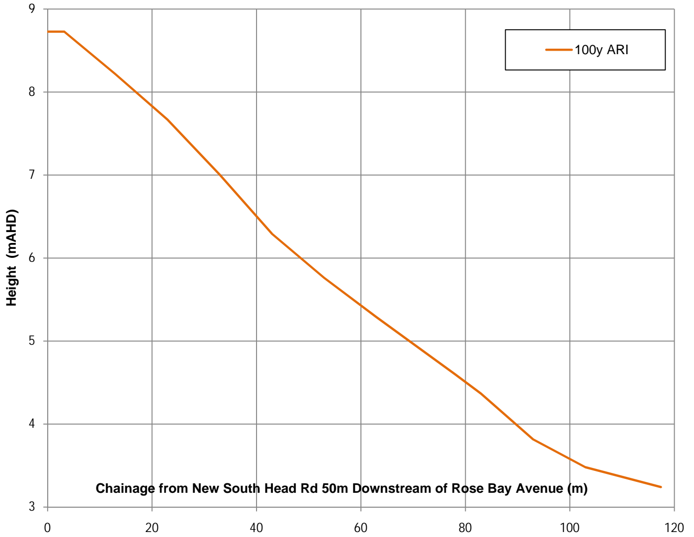
FIGURE 7j PEAK HEIGHT PROFILES REACH 10
