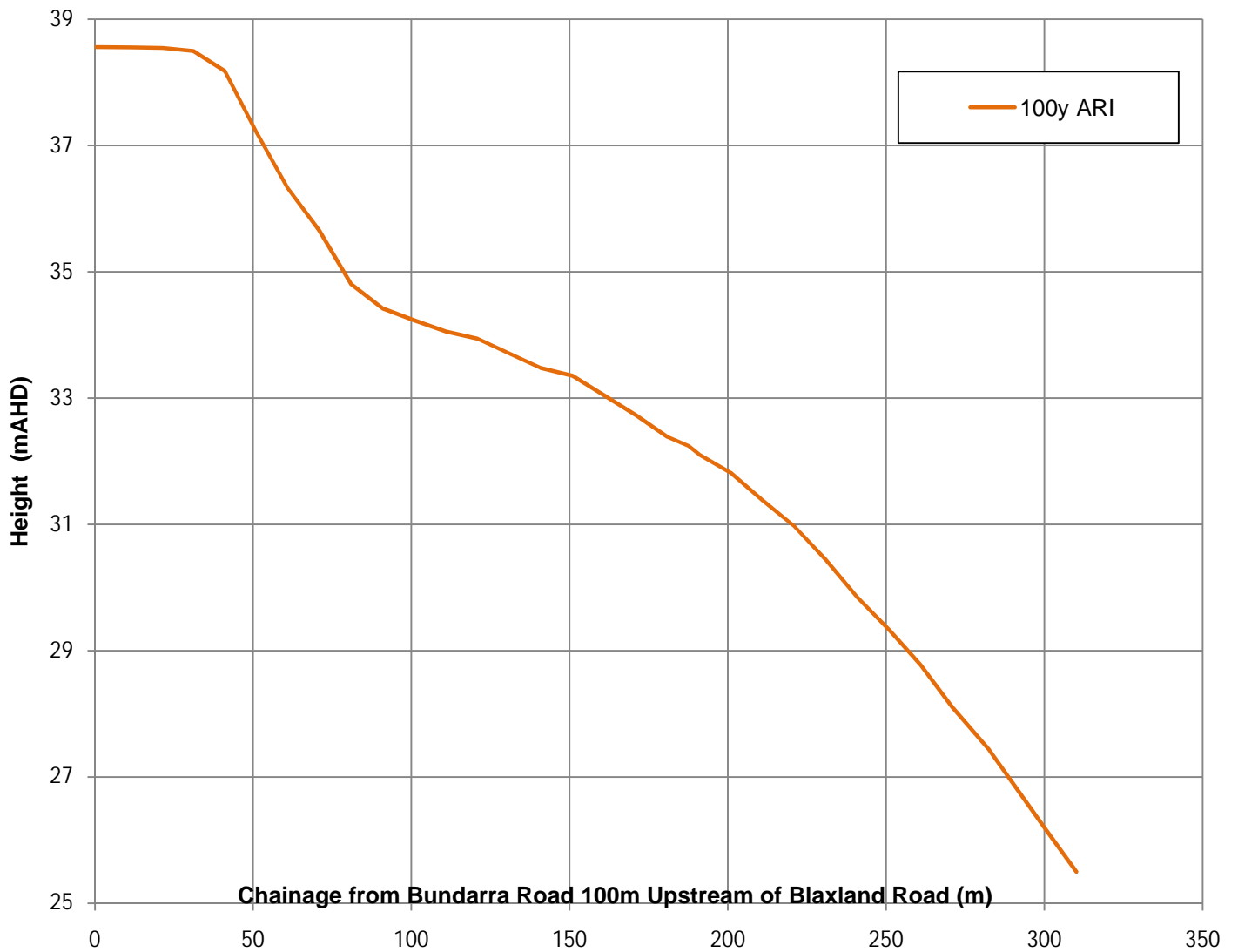
FIGURE 7d PEAK HEIGHT PROFILES REACH 4
