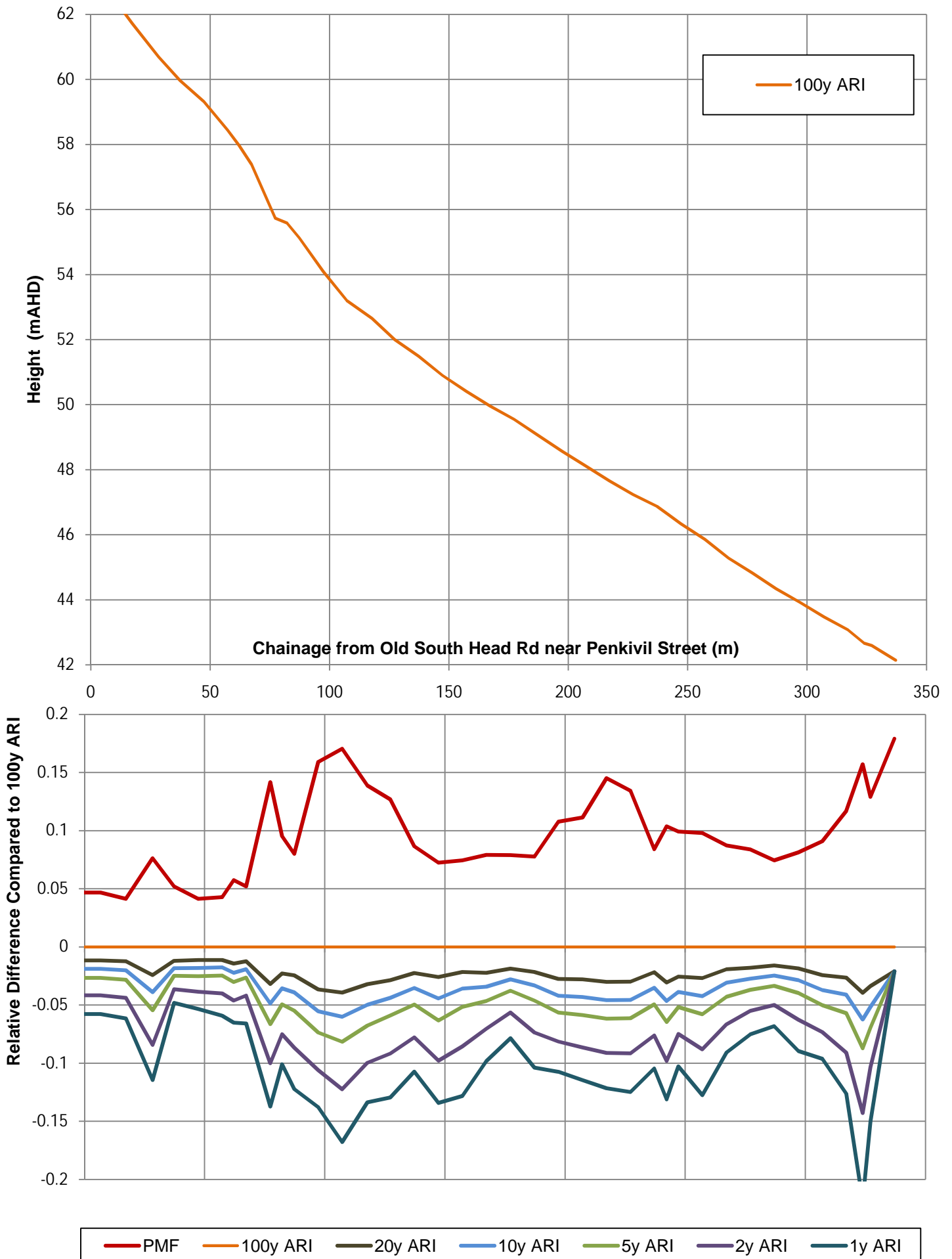
FIGURE 7c PEAK HEIGHT PROFILES REACH 3
