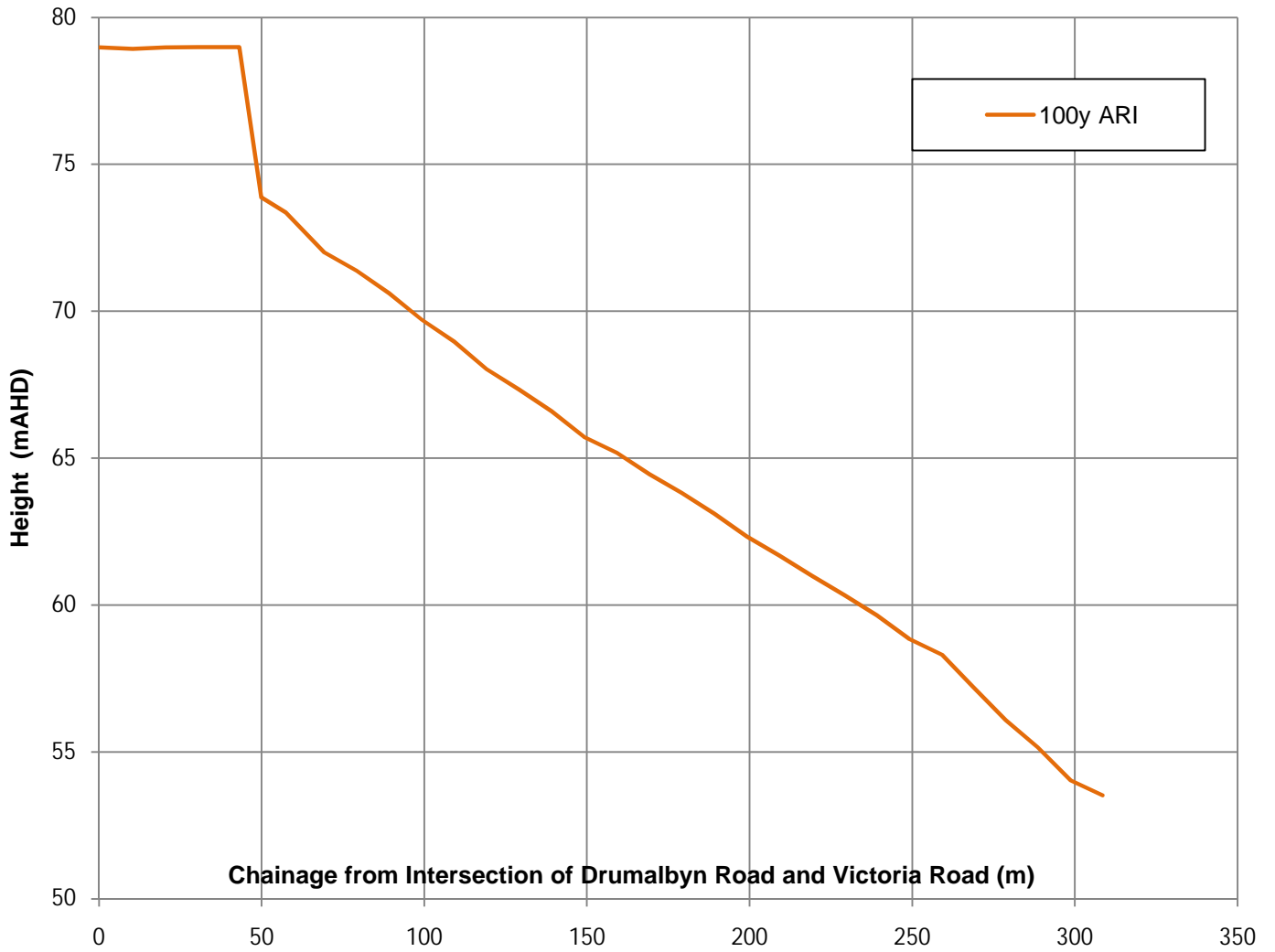
FIGURE 7g PEAK HEIGHT PROFILES REACH 7
