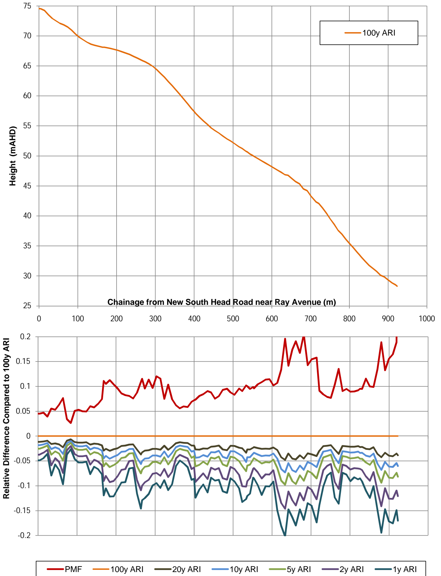
FIGURE 7a PEAK HEIGHT PROFILES REACH 1
