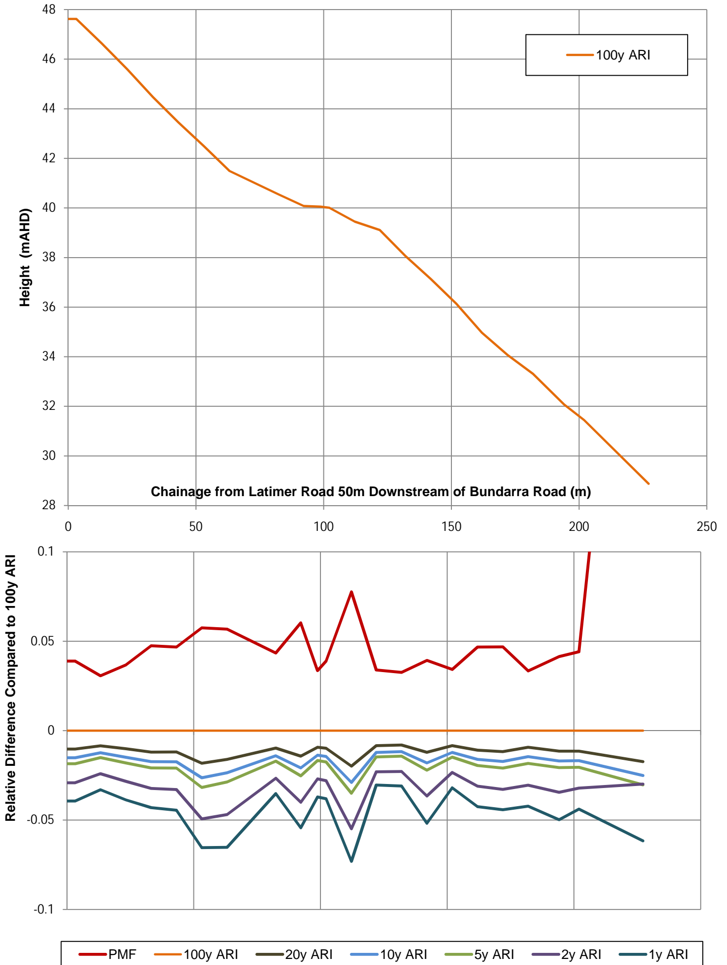
FIGURE 7f PEAK HEIGHT PROFILES REACH 6
