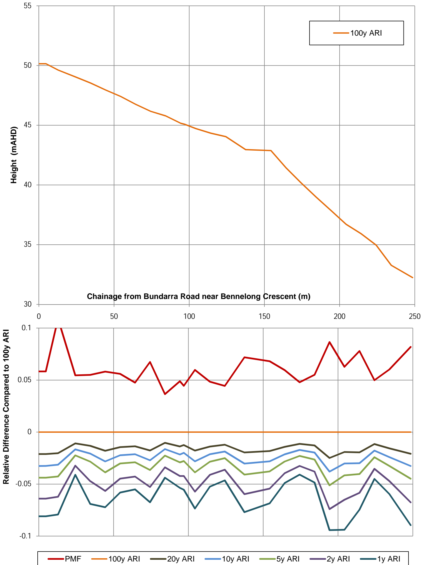
FIGURE 7e PEAK HEIGHT PROFILES REACH 5
