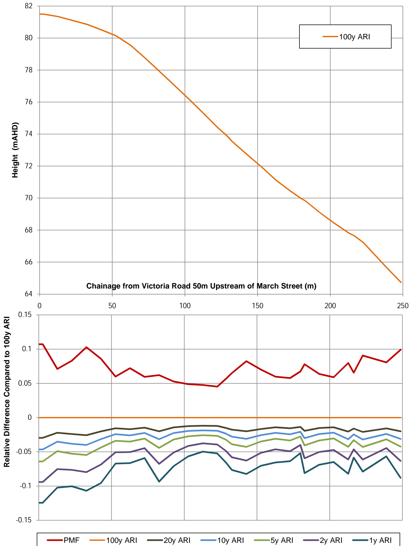
FIGURE 7h PEAK HEIGHT PROFILES REACH 8
