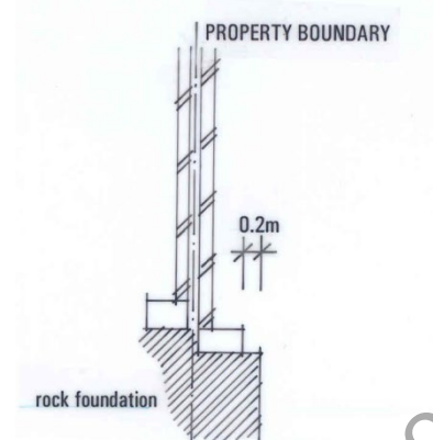
Freestanding boundary wall
