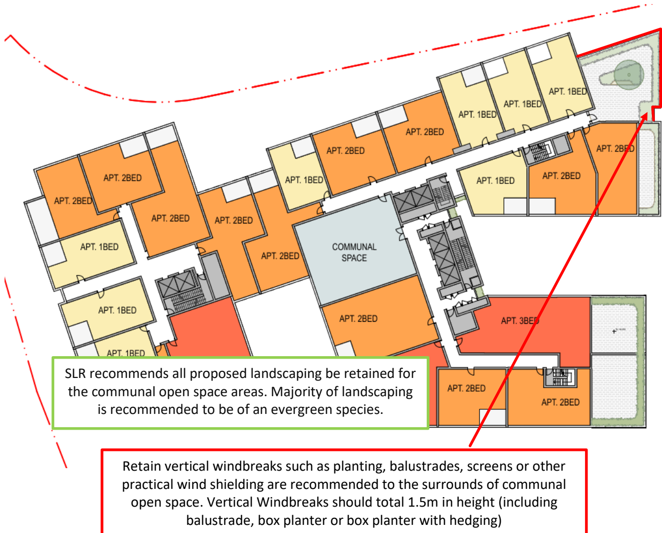
Figure 17 Mitigation Recommendations – Levels 3
