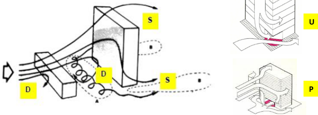
Figure 6 Wind Flow Patterns Past Regular Shaped Buildings
