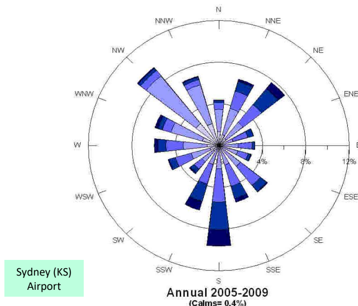
Figure 4 Annual Wind Roses for Sydney (KS) Airport (BoM Data)
