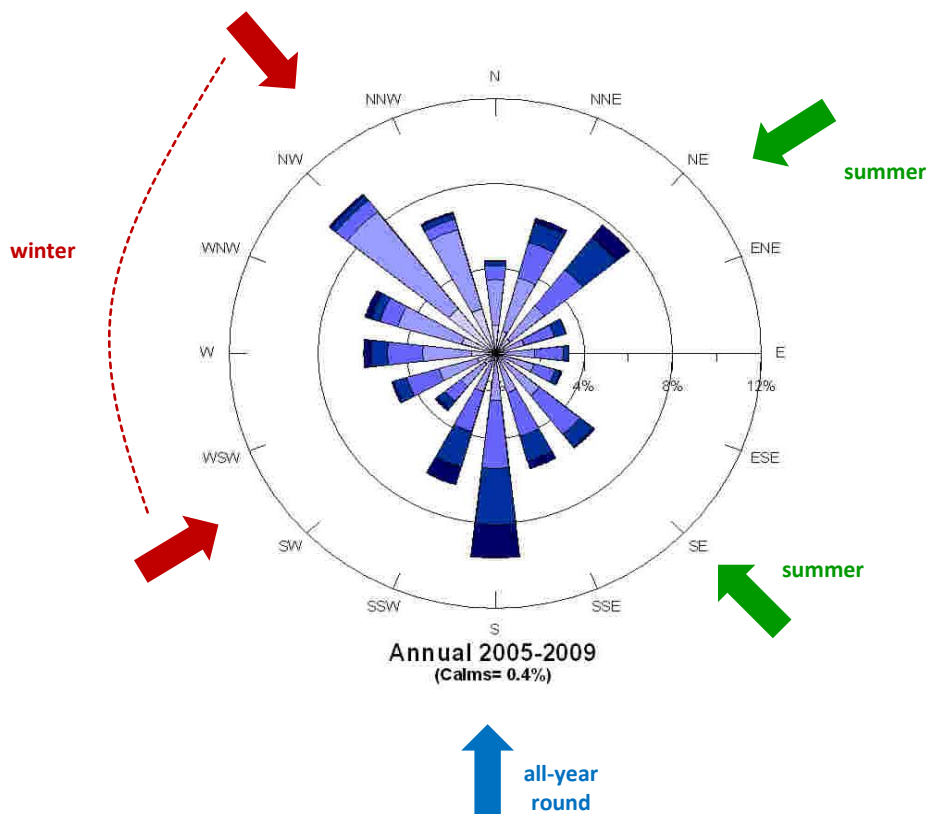
Figure 5 Seasonal Variation of Wind Speeds Expected at Edgecliff
