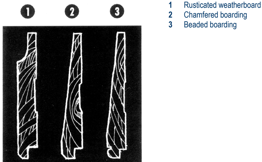
FIGURE 28 Traditional cladding profiles
