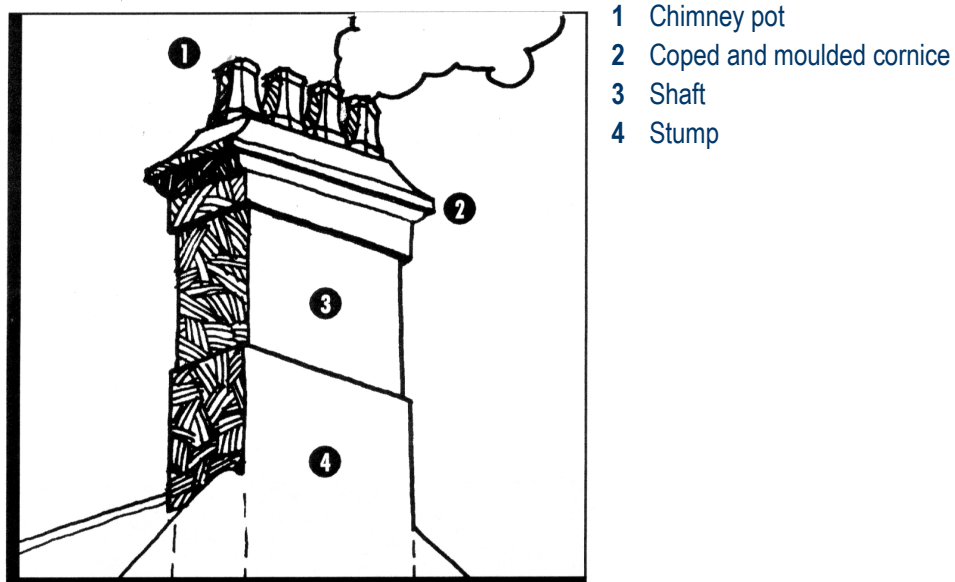
FIGURE 15 Typical chimney stack
