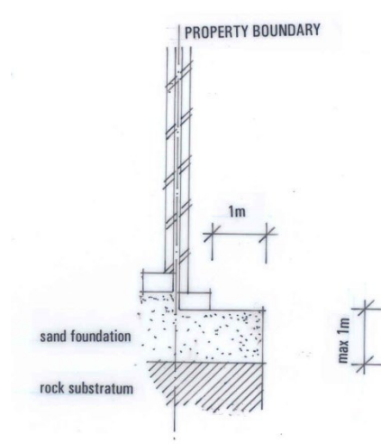
Freestanding boundary wall
