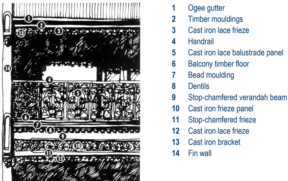
FIGURE 18 Verandahs and balconies
