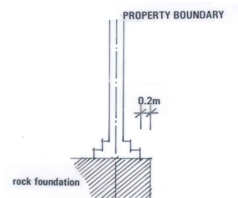
Common party wall
