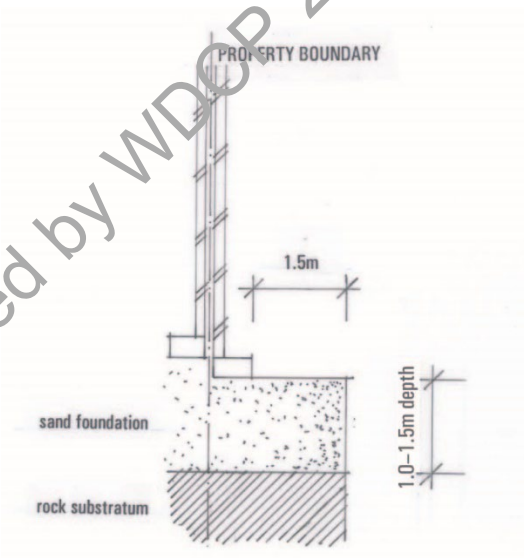
Common party wall
